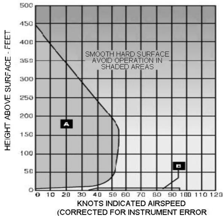
Figure III-15-4. Height-velocity diagram
