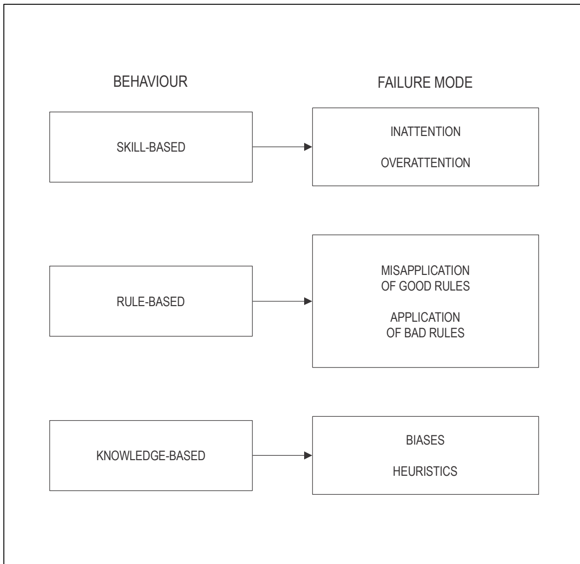
Figure III-16-14. Breakdown of behaviour into failure modes
