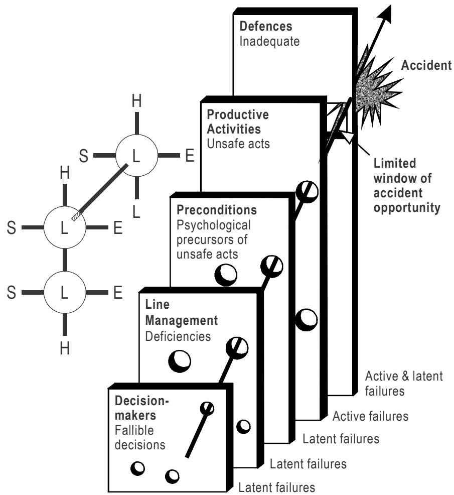
Figure III-16-6. SHEL and Reason hybrid model
