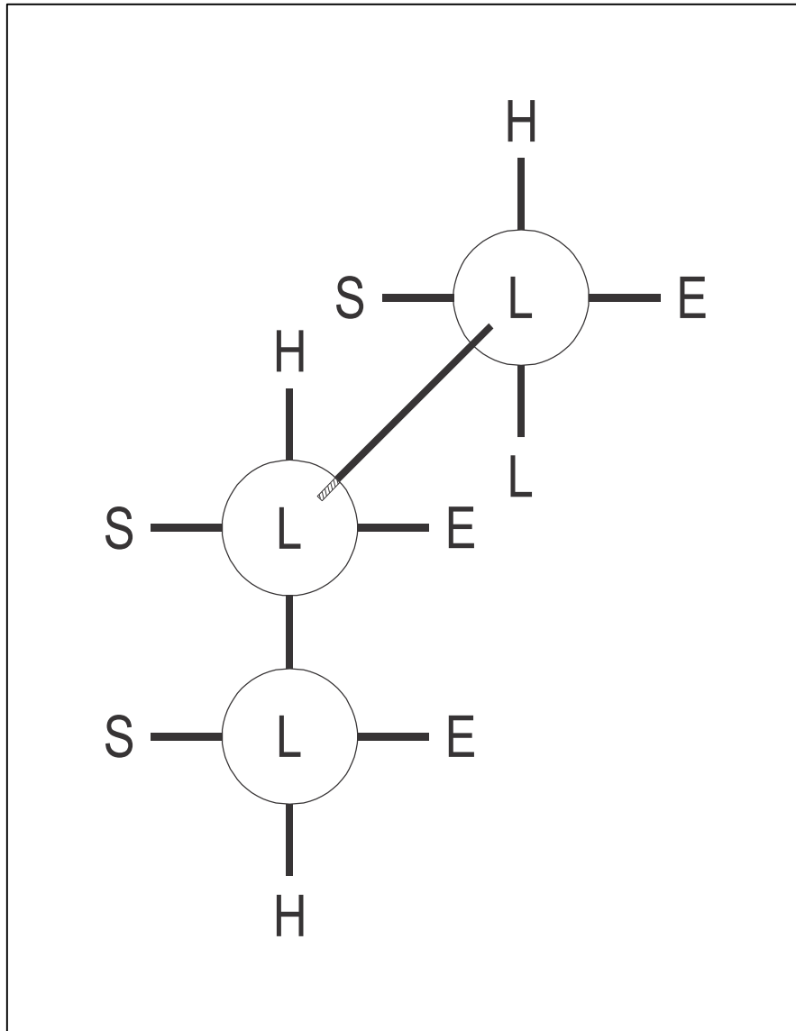
Figure III-16-11. Modified SHEL model
