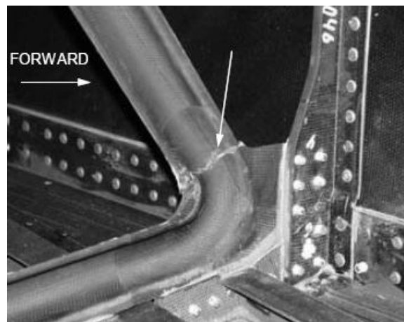
Figure III-9-53. Several carbon fibre composite reinforced components of the A300-600s vertical tail are joined with fasteners in single- and double-row fastener patterns. White arrow indicates structural failure.
