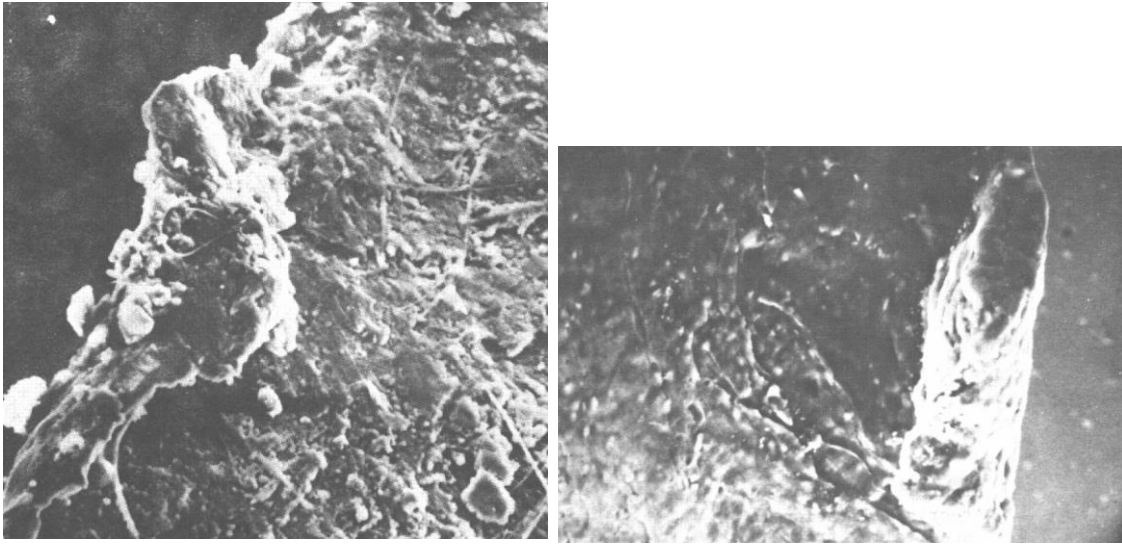
Figure III-19-7. (Left) Rolled edge effect on a fragment from the Comet aircraft; (Right) Controlled detonation of NG-based explosive in association with a zinc-based 1.5 volt dry cell
