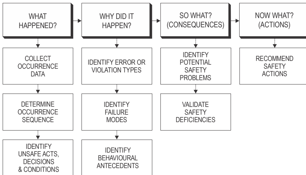
Figure III-16-10. Investigation functions and component task activities
