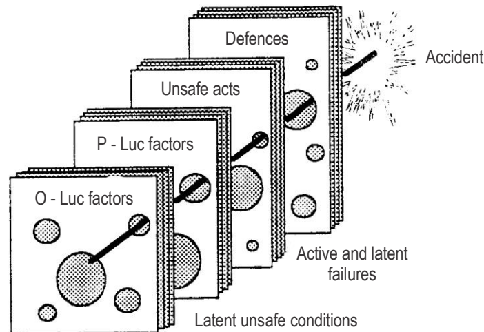
Figure III-16-3. Latent unsafe conditions within the Reason framework
