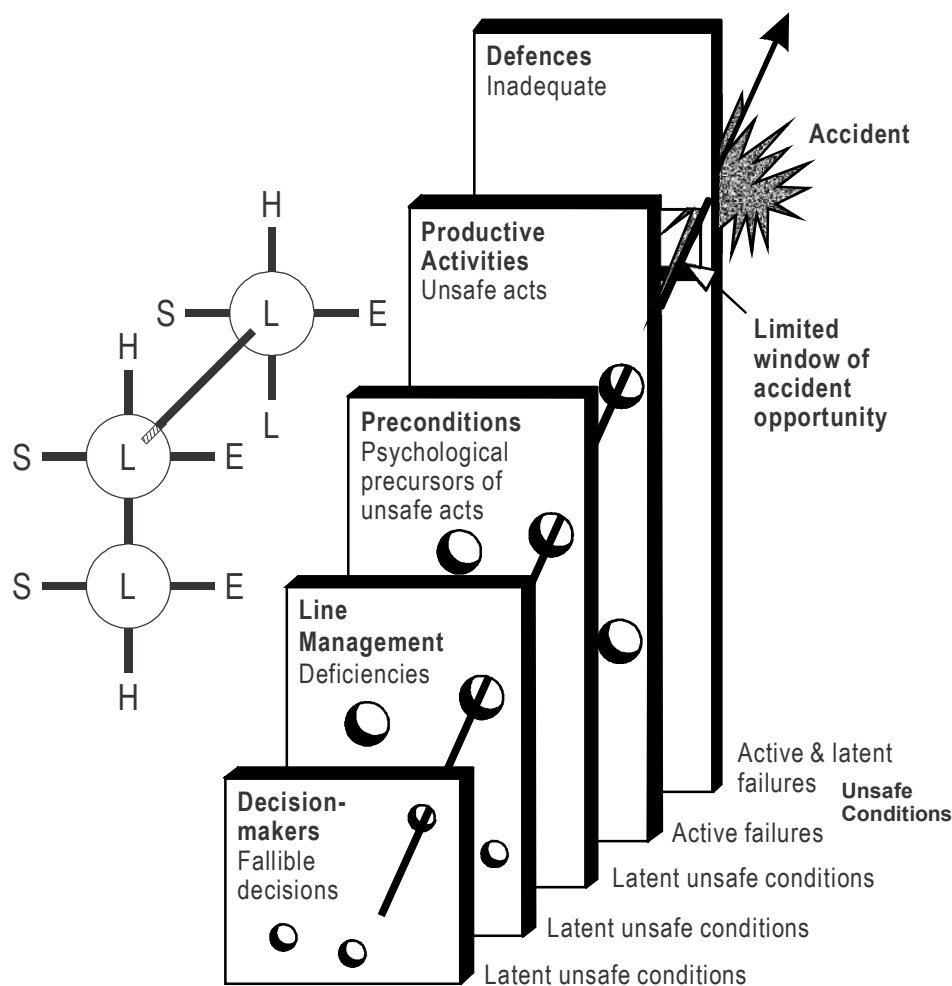
Figure III-16-12. SHEL and Reason hybrid model
