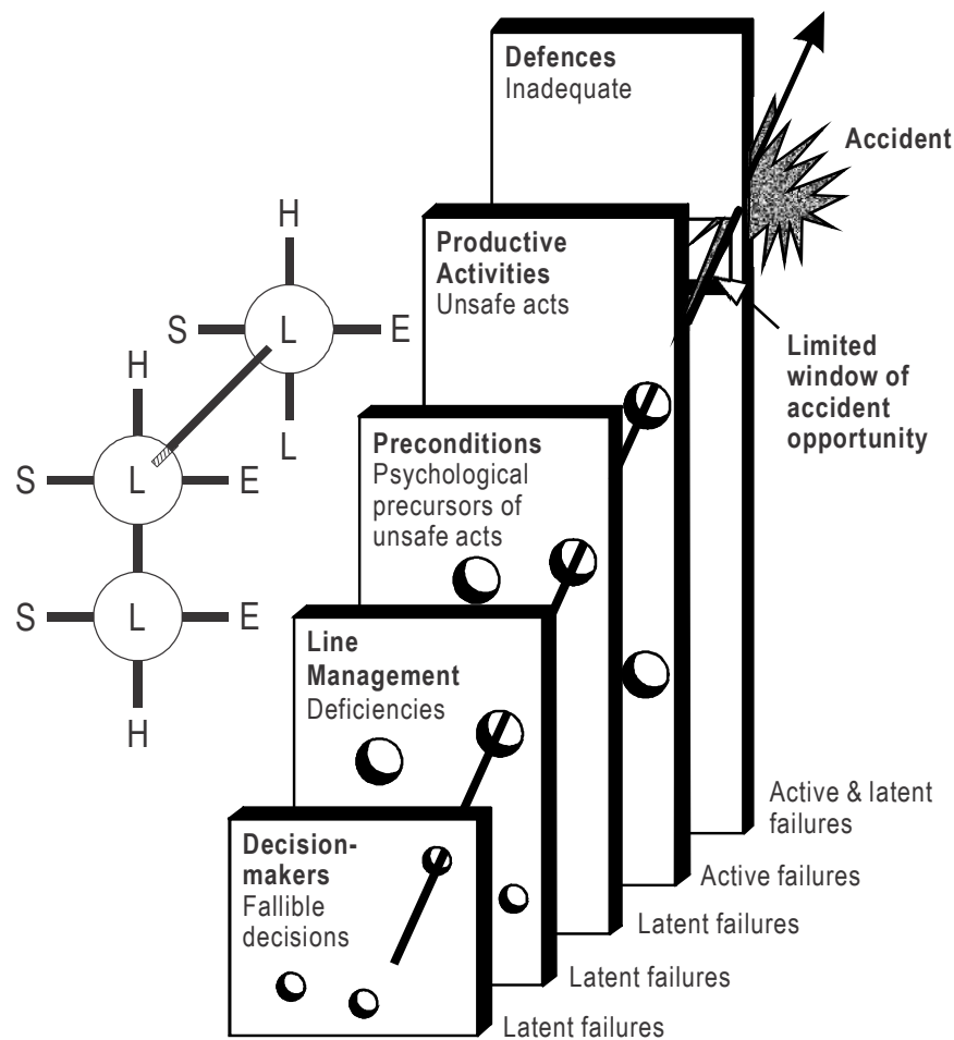
Figure III-16-7. The GEMS Framework (adapted from Reason, 1990)
