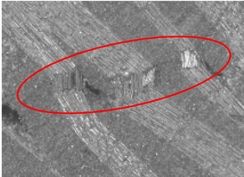
Figure III-9-29. Example of fibre kinking as a result of compressive loads
