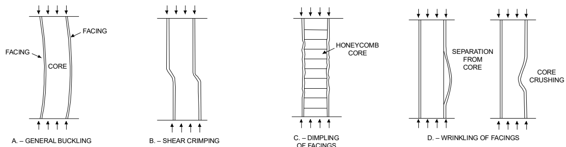
Figure III-9-41. Compression failures in sandwich beams
