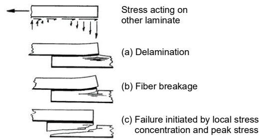
Figure III-9-48. Potential failure modes of simple bonded lap joints
