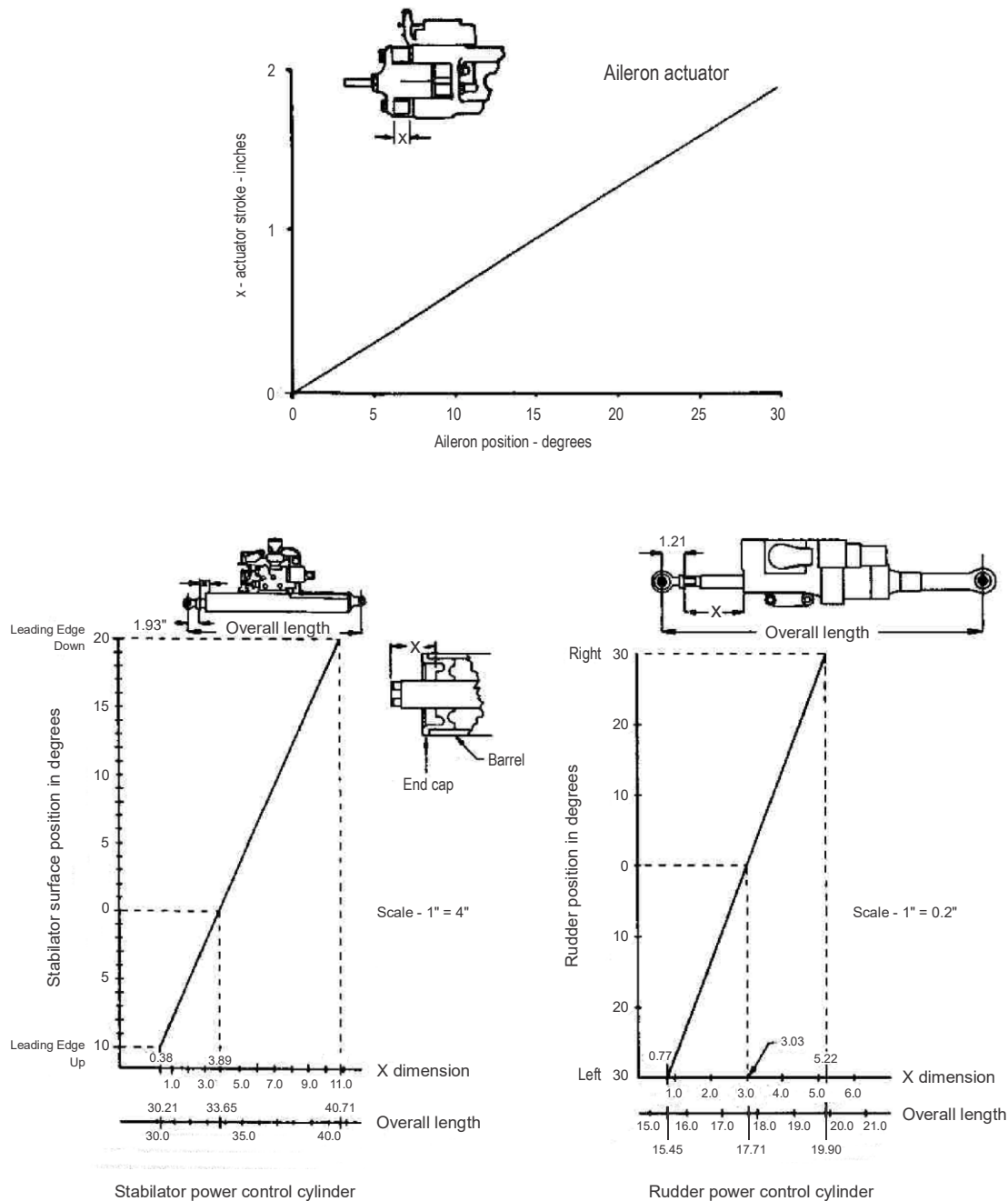
Figure III-13-1. Evaluating actuator position
