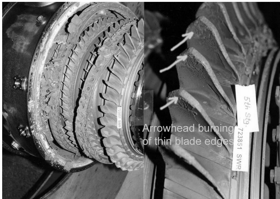
Figure III-12-26. Titanium fire damage (note arrowhead effect)
