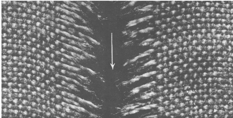
Figure III-9-14. Tearing. Fibres turned in the direction of propagation of failure.
