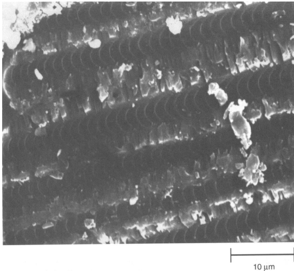
Figure III-9-34. Striations at the interface between fibres and matrix
