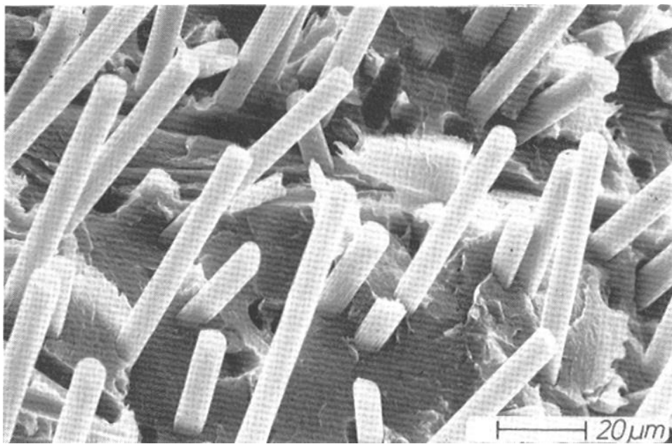
Figure III-9-28. Example of fibre pullout as a result of tensile loads
