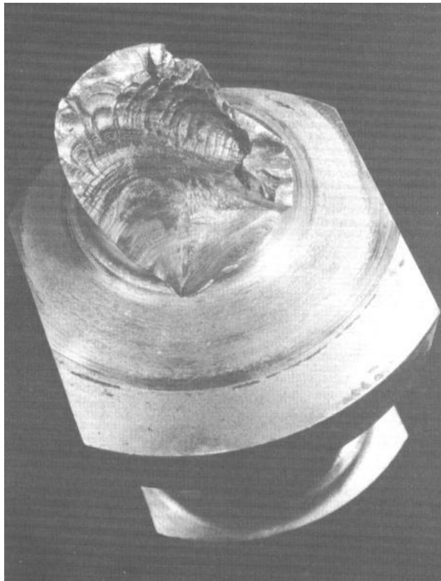
Figure III-9-7. Fatigue failure of a punch press shaft which was subjected to torsion and bending loads. The fatigue crack originated at a sharp fillet at a change in section.
