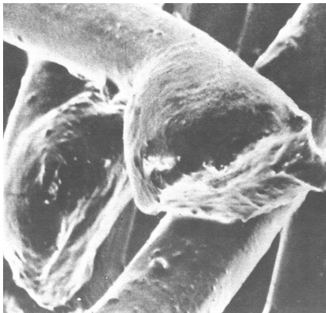
Figure III-19-18. Globularized ends of fibres showing absence of blackening and gas bubbles
