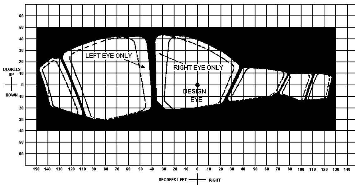
Figure III-4-1. Captain design eye and ambinoocular vision areas. Shaded areas represent structure and are not visible with either eye unless the captain moves from the normal design eye position.
