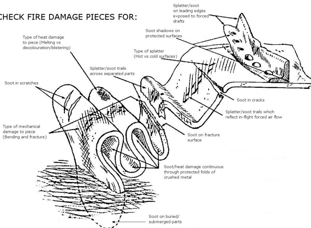
Figure III-11-2. Evaluating fire damage on wreckage
