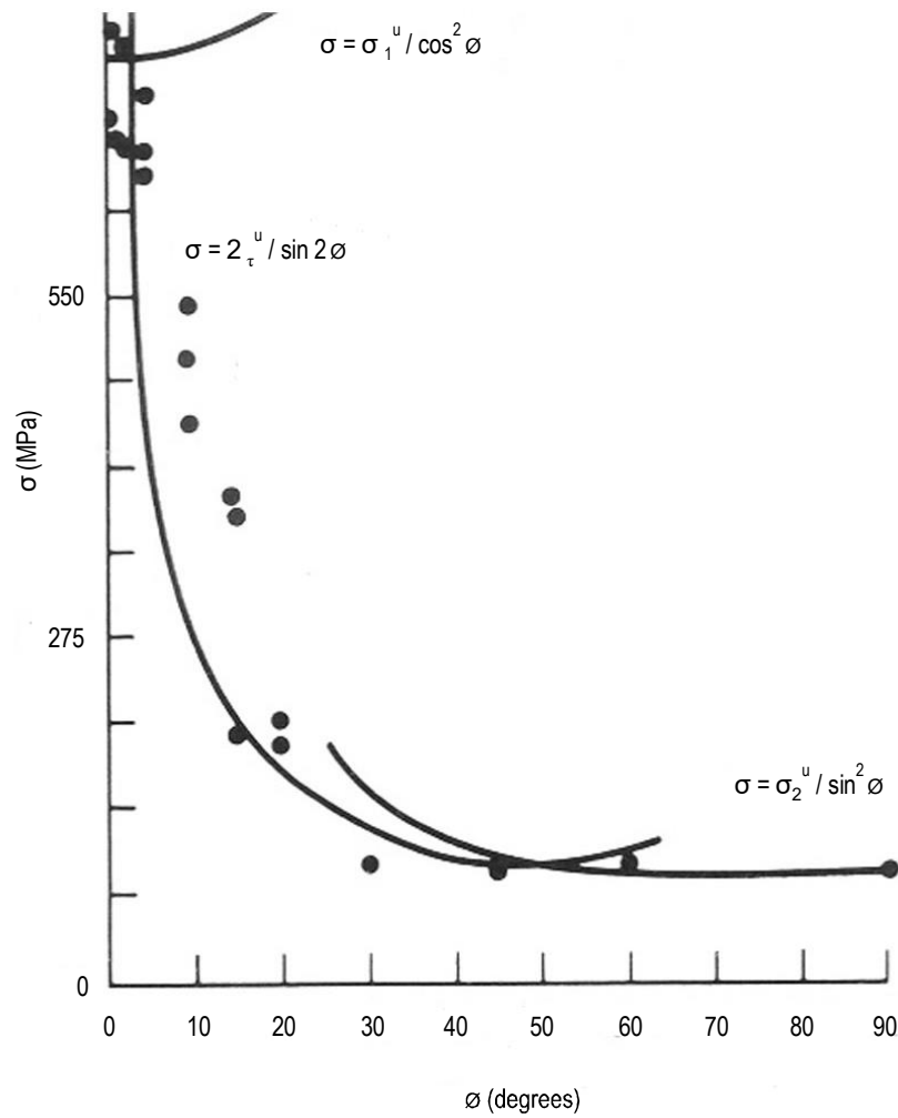
Figure III-9-26. The strength of a single unidirectional composite ply, based on the angle between the fibres and the loading direction, where \sigma_1^u is the measured ultimate strength of the laminate along the fibre direction, \sigma_2^u is the measured ultimate strength of the laminate perpendicular to the fibre direction, and \tau^u is the measured ultimate shear strength of the laminate.
