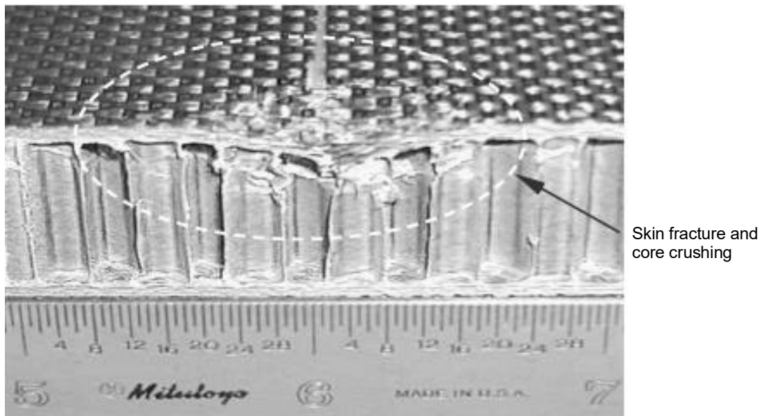
Figure III-9-44. Crushed core and fractured face sheet
