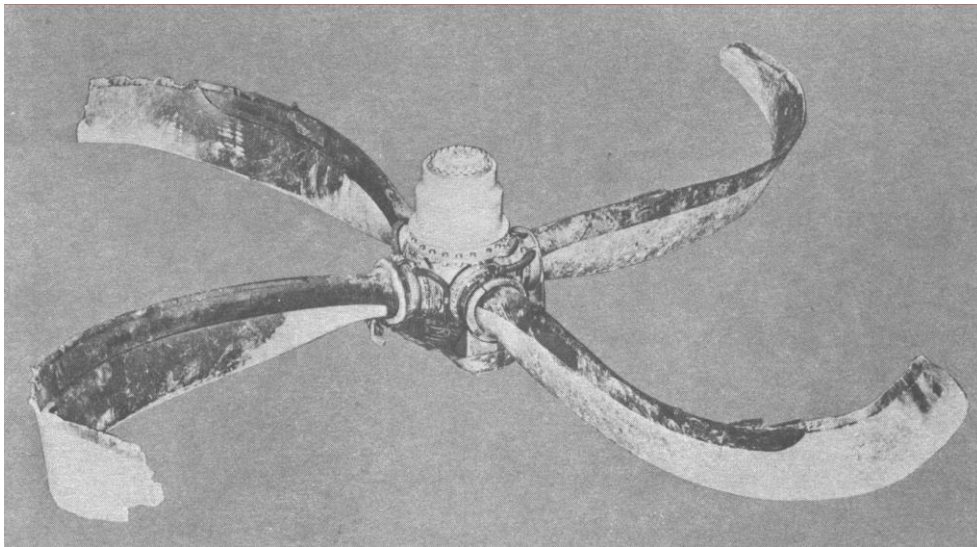
Figure III-12-30. Metal propeller under power at impact
