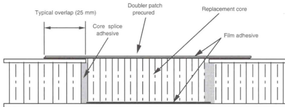
Figure III-9-60. Adhesively fastened patch repair in a sandwich structure cross-section, similar to the repair shown in Figure III-9-59
