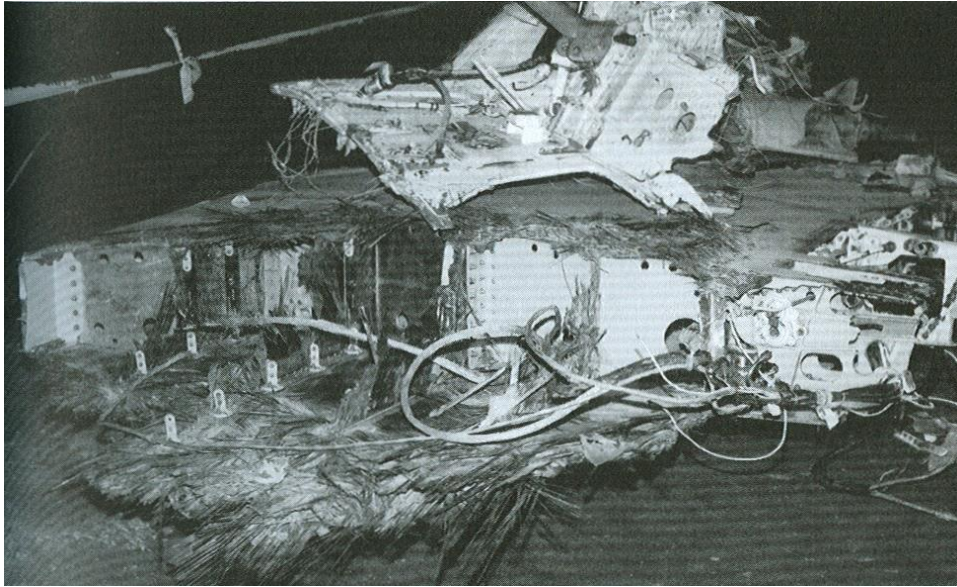
Figure III-9-32. Composite wing that reportedly failed in bending. The relatively rough area of tension failure with significant fibre pullout and the relatively smooth area of compression failure are clearly identifiable.
