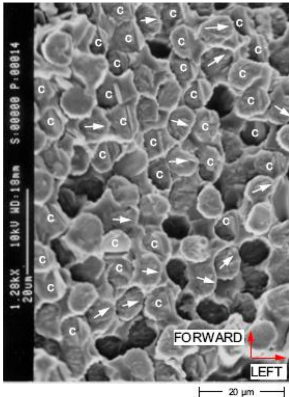
Figure III-9-36. Fractures in multiple locations exhibited chop marks (marked with a “c”) on the ends of fractured fibres, consistent with compressive loading and buckling of fibres.
