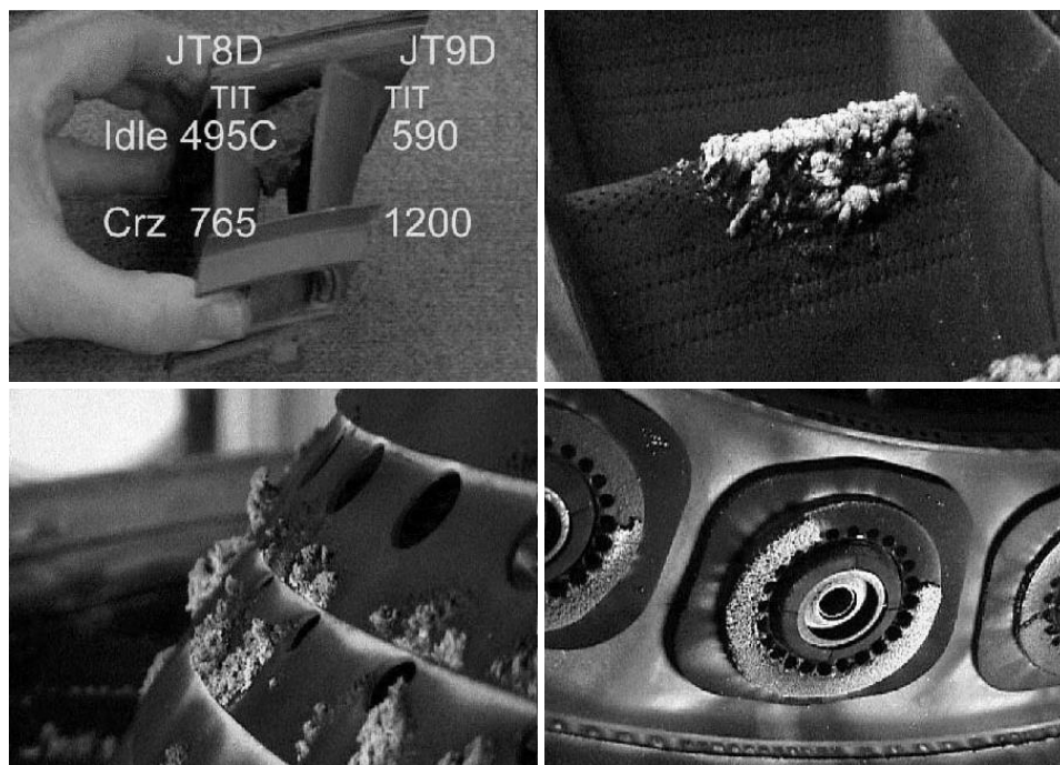
Figure III-12-20. Volcanic ash melted and adhering to hot section parts
