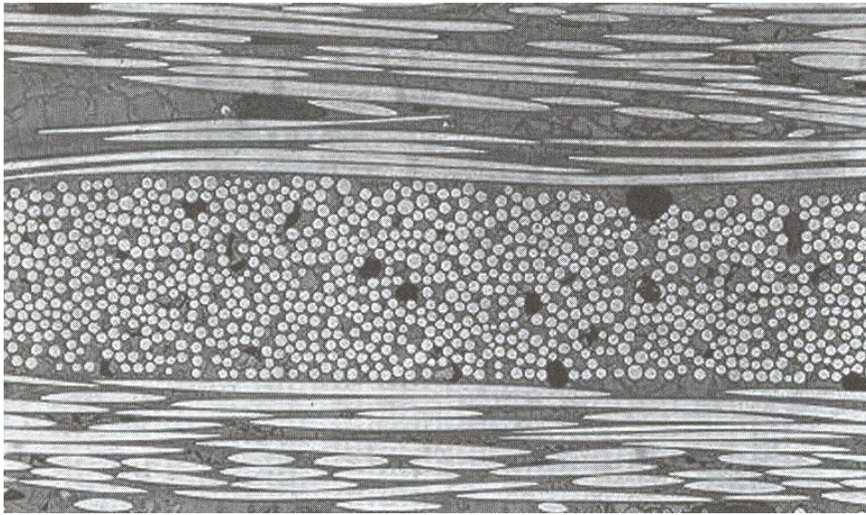
Figure III-9-27. Laminate cross-section indicating the ply-wise variation in fibre orientation
