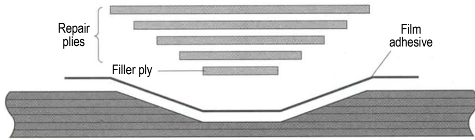
Figure III-9-61. Adhesively bonded patch with a scarf interface in a laminate
