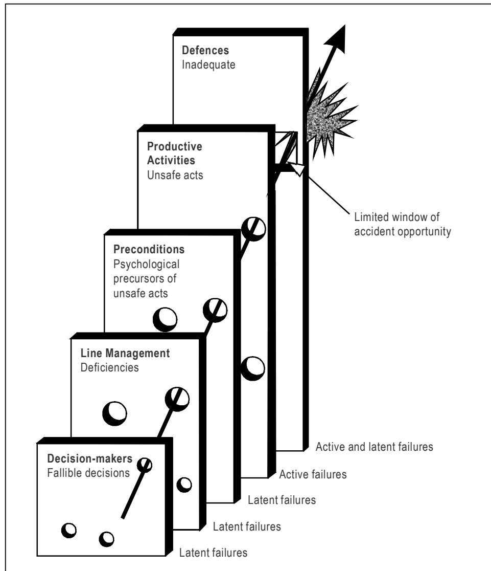
Figure III-16-2. Reason's model Latent Unsafe Conditions (LUC) framework
