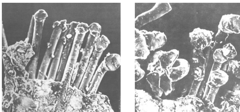
Figure III-19-19. (Left) Controlled-explosion damage to Canadian Nylon 66 sample; (Right) Enlarged view
