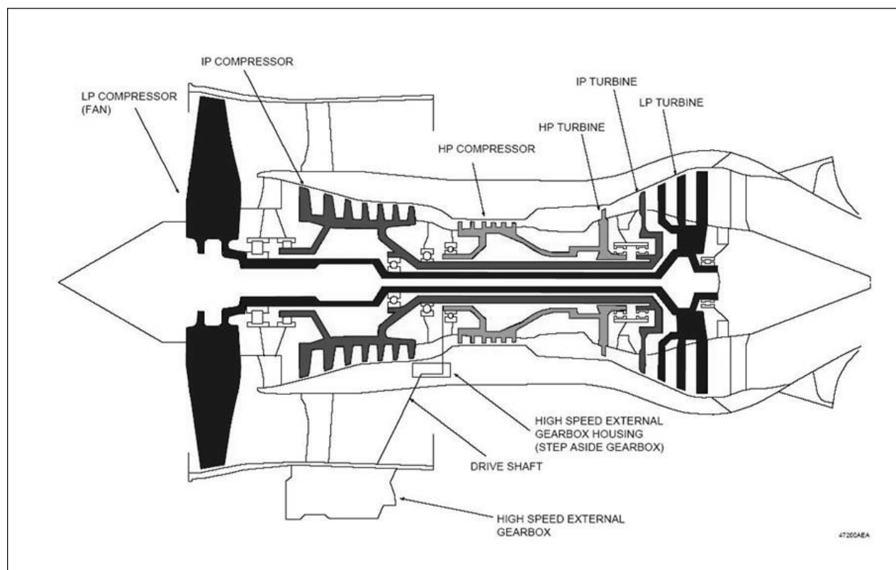
Figure III-12-1 A typical large transport engine
