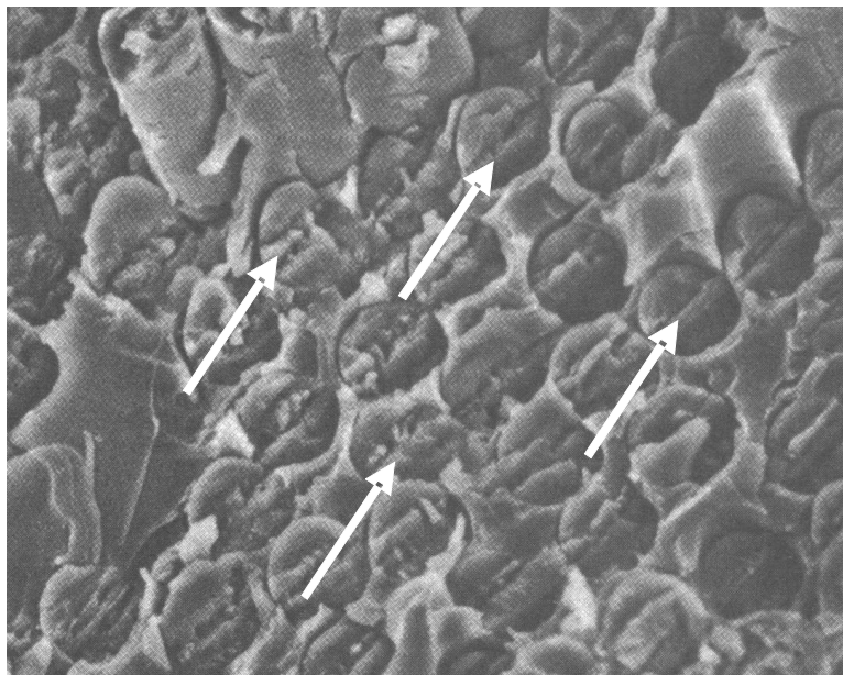
Figure III-9-30. Chop marks can be produced on the ends of broken fibres that have buckled and failed under compressive loads.
