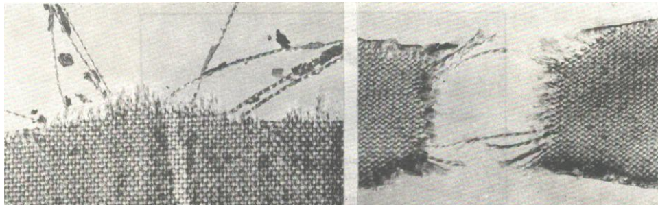
Figure III-9-13. Fabric failures in tension. Left: Bushy appearance, fibres straight along threads. Right: Bushy appearance, fibres turned locally at fracture across threads.
