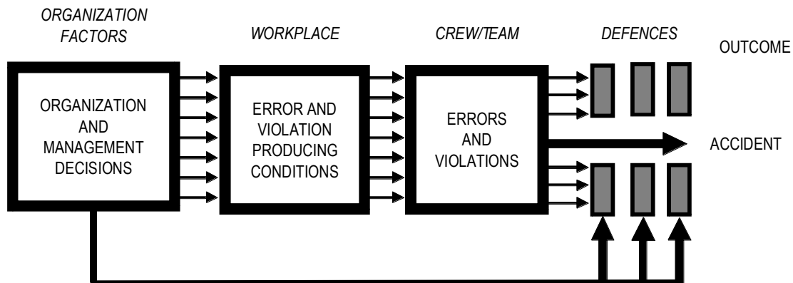
Figure III-3-1 Accident causation model (Adapted from Prof. James Reason)
