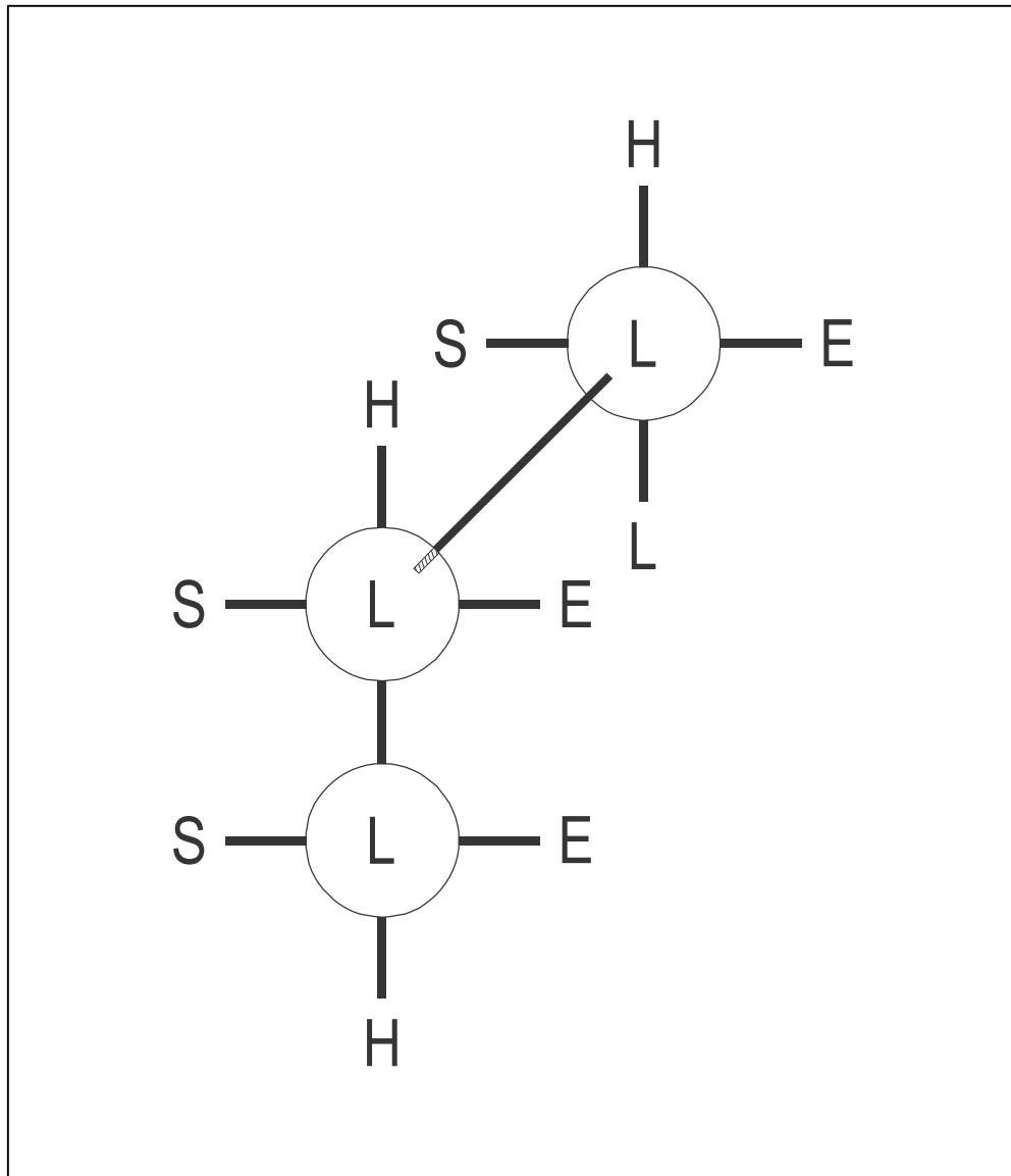
Figure III-16-5. Modified SHEL Model
