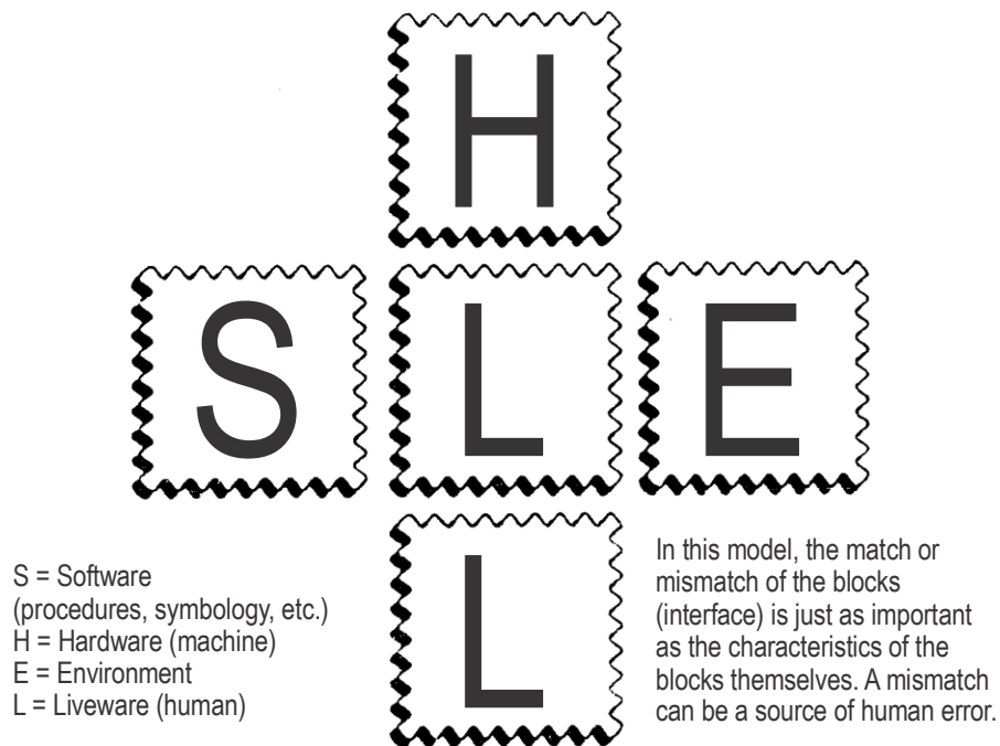
Figure III-16-1. The SHEL model (adapted from Hawkins, 1975)
