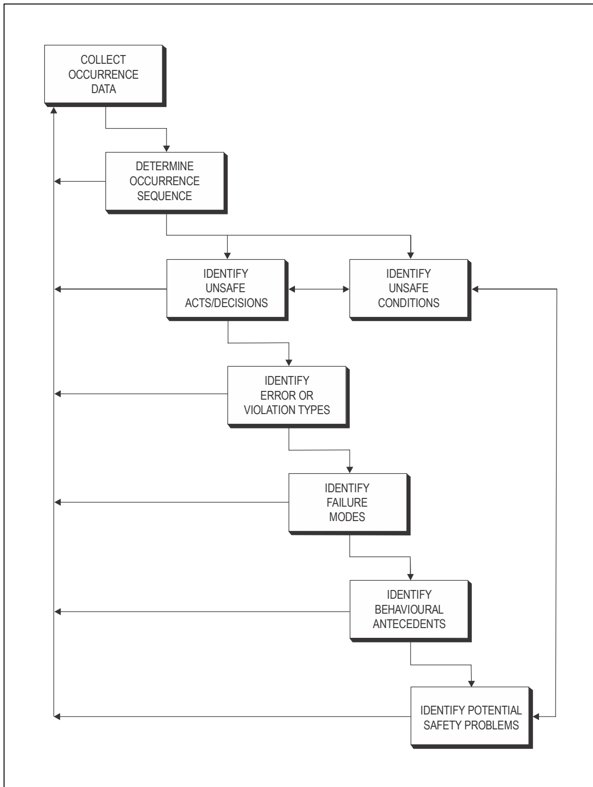
Figure III-16-9. An integrated process for occurrence investigation
