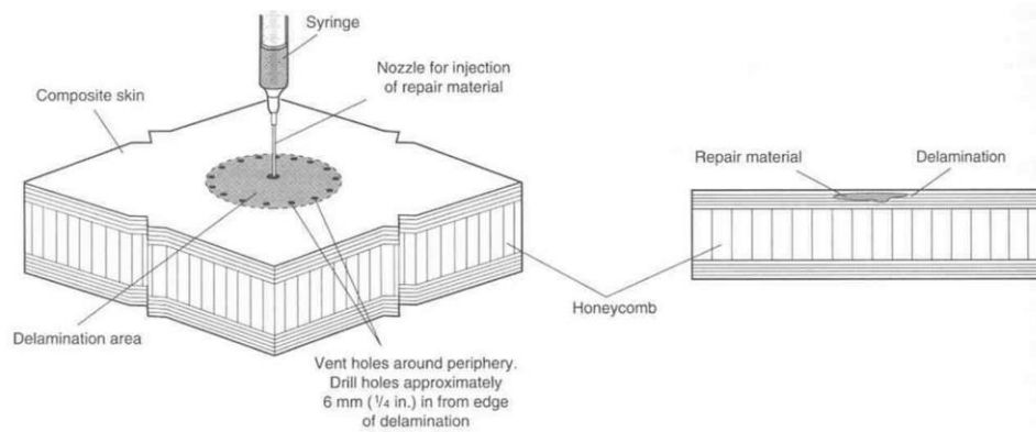
Figure III-9-65. The delamination on the right side is repaired with the resin injection procedure demonstrated on the left side.
